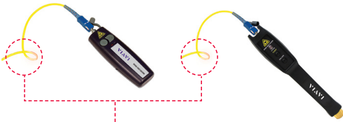
Red illumination indicating fiber damage/bend
