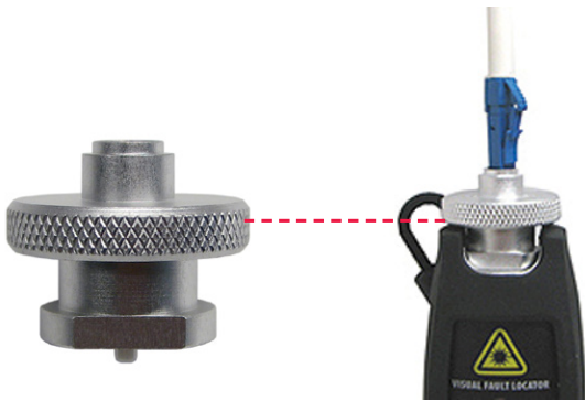
Universal 1.25 mm adapter for FFL-100
